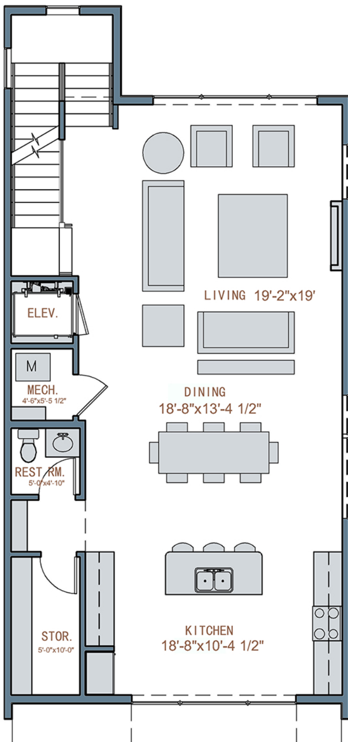
THIRD FLOOR 1033 SQ. FT.
